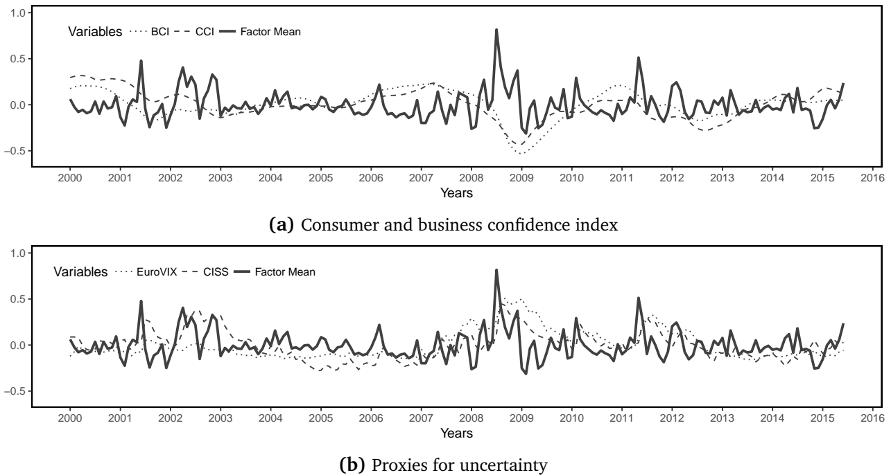
Fig. 2: Comparison of the estimated uncertainty factor and other measures.
